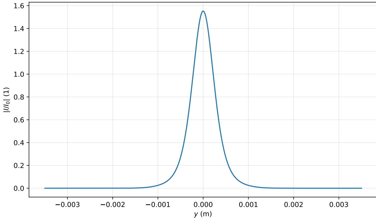
Intensity profile I(x=0, y, z=1.433)/I_0 , P_{in}=0.9P_{cr} , artificial time
